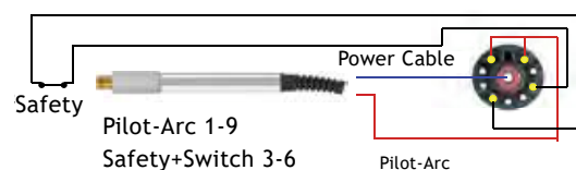
Machine Torch XM 160
