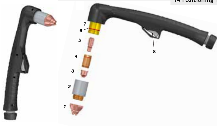
Plasma torch XT 160
