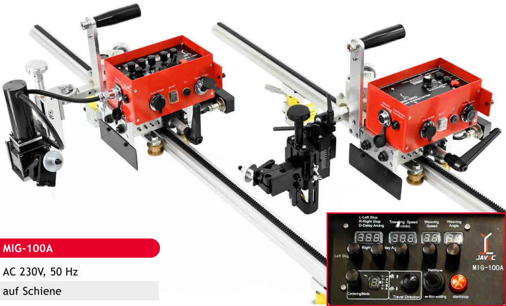
Bedienfeld MIG-100A
