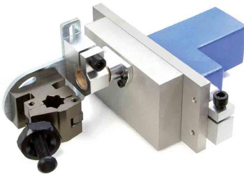
Linear-Oszillator JC-WLS
