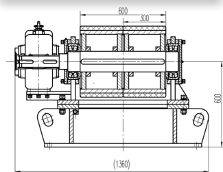
HGK-150
