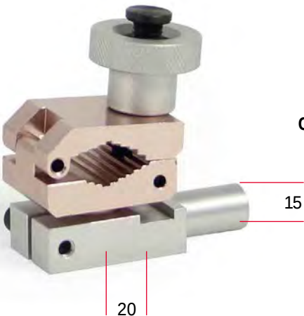
Clamp mounting Type 6
