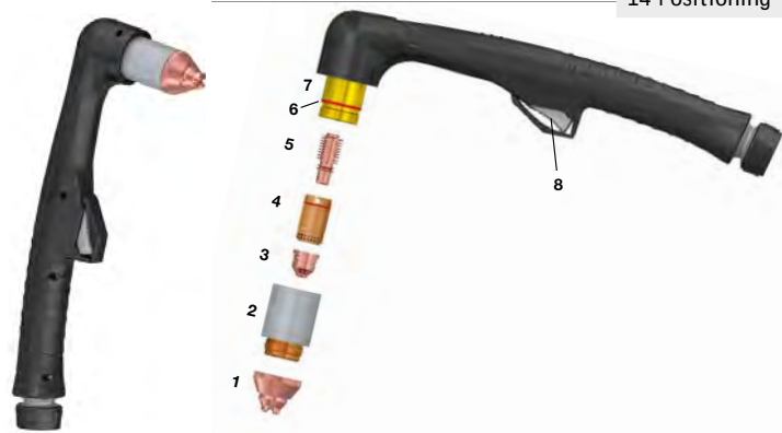
Plasma torch XT 160
