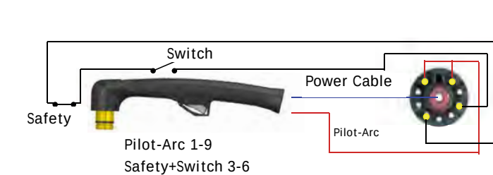
Plasma torch XT 160
