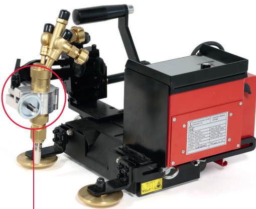
Attachement for cutting torch, Item no. 02.20.02.10020
